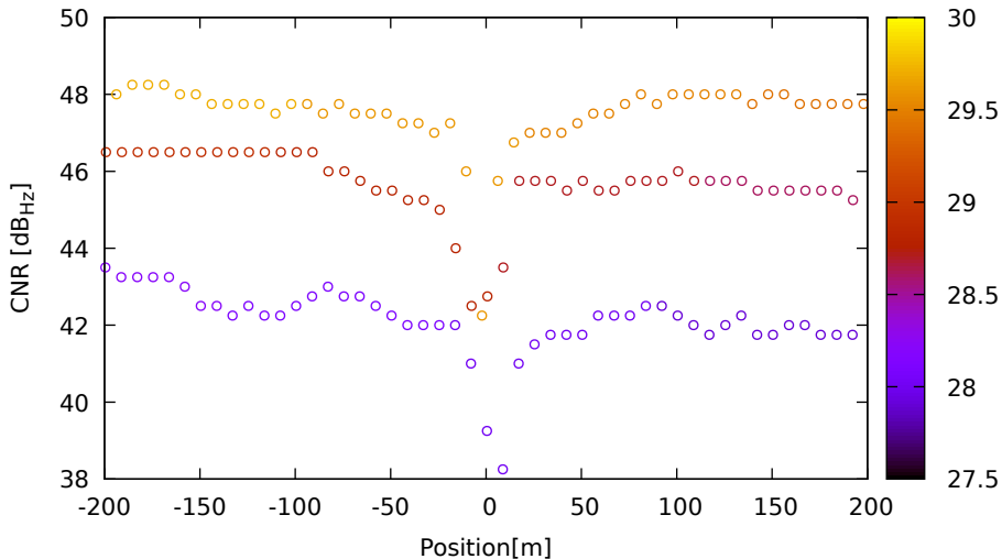
CNR vs position for C11 (B1) on SamsungS20 - DOY 263 jam. 3
