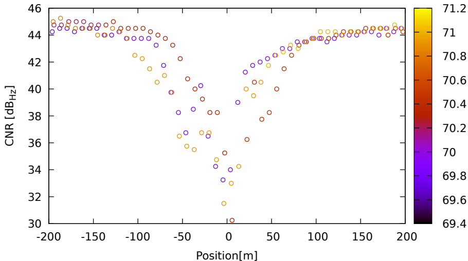
CNR vs position for C14 (B1) on SamsungS20 - DOY 263 jam. 1
