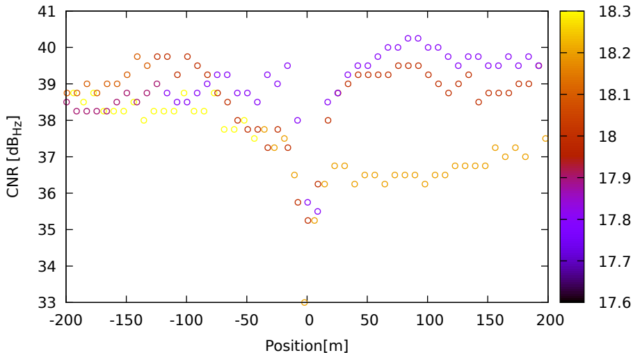
CNR vs position for C16 (B1) on SamsungS20 - DOY 263 jam. 3
