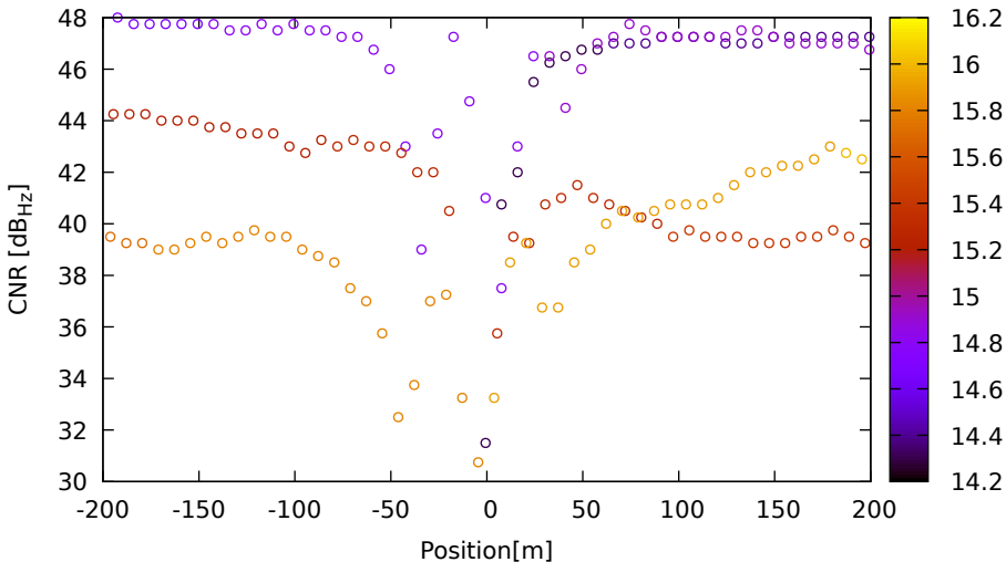
CNR vs position for C26 (B1) on SamsungS20 - DOY 263 jam. 2
