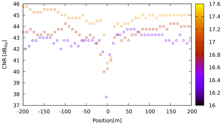
CNR vs position for C26 (B1) on SamsungS20 - DOY 263 jam. 3
