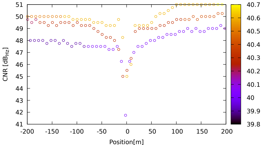
CNR vs position for C28 (B1) on SamsungS20 - DOY 263 jam. 3
