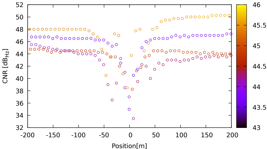
CNR vs position for C33 (B1) on SamsungS20 - DOY 263 jam. 2
