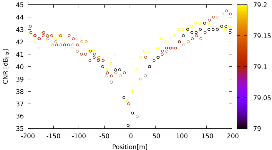
CNR vs position for E10 (E1) on SamsungS20 - DOY 263 jam. 1
