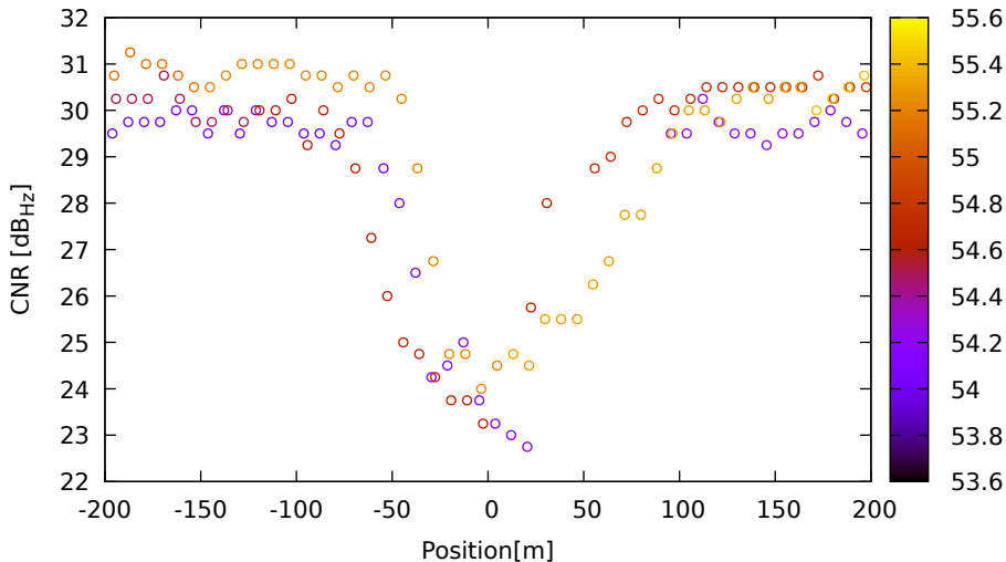
CNR vs position for E11 (E5a) on SamsungS20 - DOY 263 jam. 1
