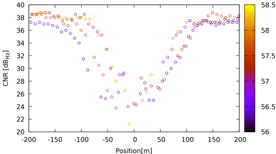
CNR vs position for E19 (E1) on SamsungS20 - DOY 263 jam. 2
