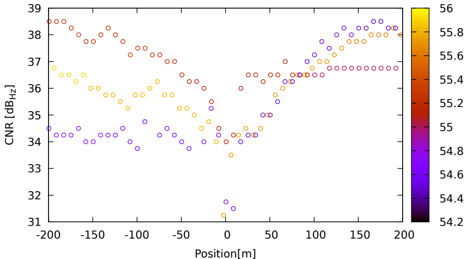
CNR vs position for E19 (E1) on SamsungS20 - DOY 263 jam. 3
