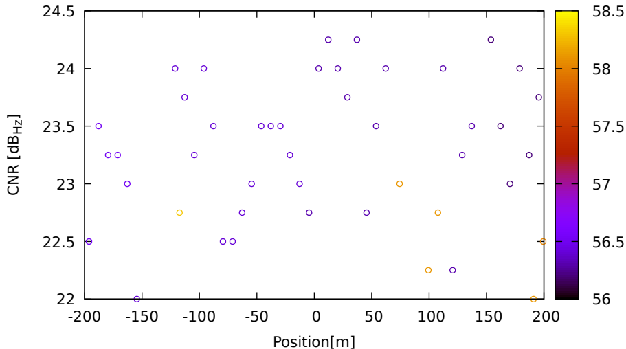
CNR vs position for E19 (E5a) on SamsungS20 - DOY 263 jam. 2
