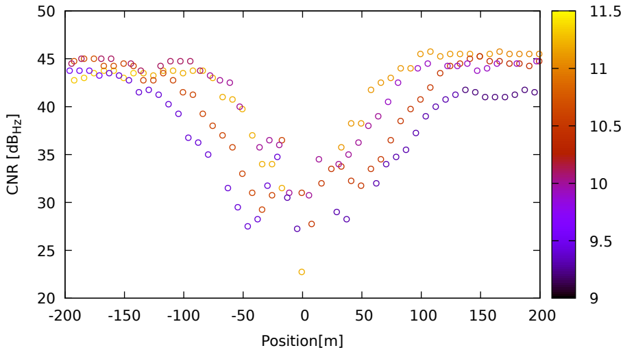
CNR vs position for E33 (E1) on SamsungS20 - DOY 263 jam. 2
