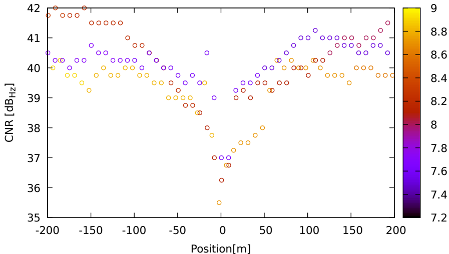
CNR vs position for E33 (E1) on SamsungS20 - DOY 263 jam. 3
