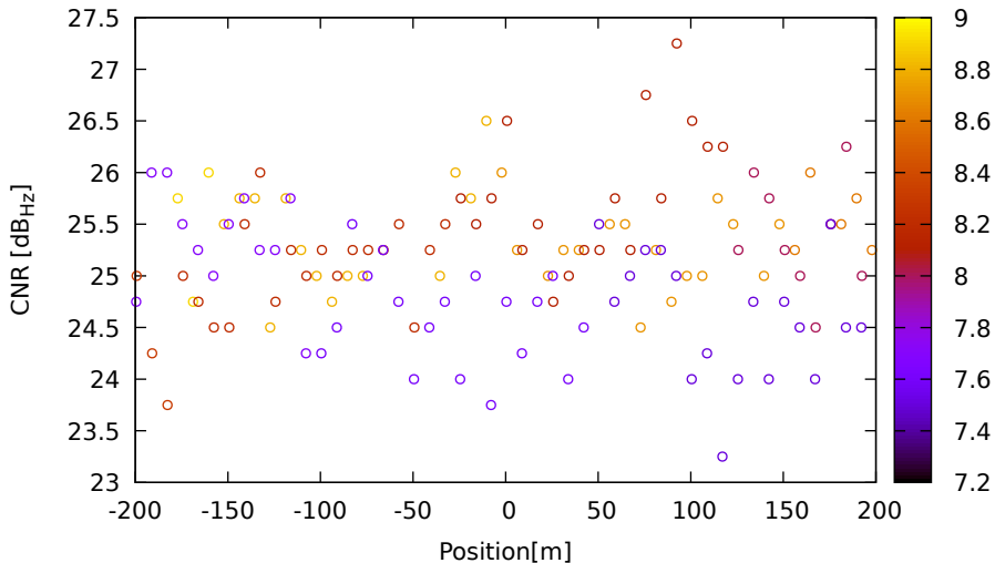
CNR vs position for E33 (E5a) on SamsungS20 - DOY 263 jam. 3
