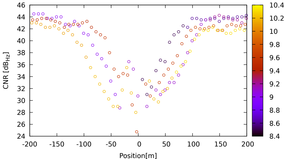
CNR vs position for E36 (E1) on SamsungS20 - DOY 263 jam. 2
