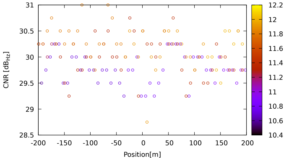
CNR vs position for E36 (E5a) on SamsungS20 - DOY 263 jam. 3
