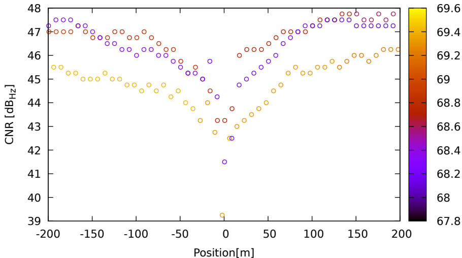
CNR vs position for G03 (L1) on SamsungS20 - DOY 263 jam. 3
