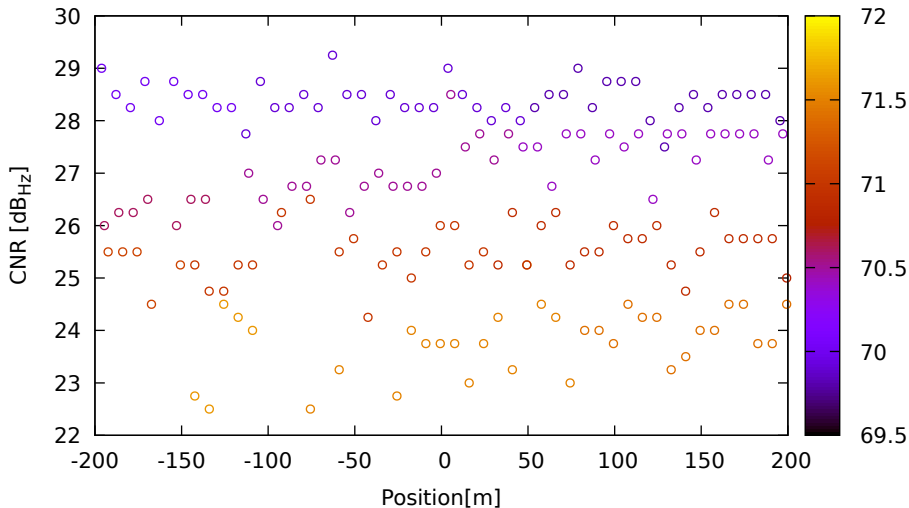
CNR vs position for G03 (L5) on SamsungS20 - DOY 263 jam. 2
