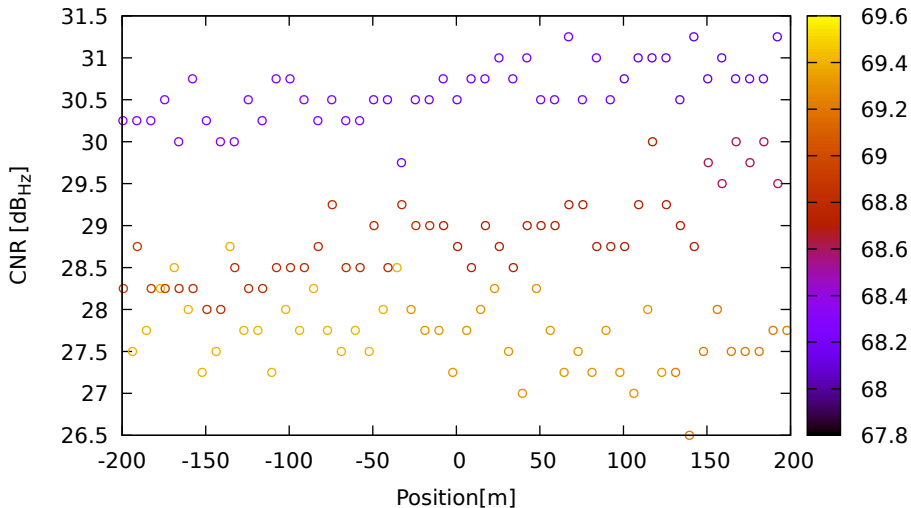
CNR vs position for G03 (L5) on SamsungS20 - DOY 263 jam. 3
