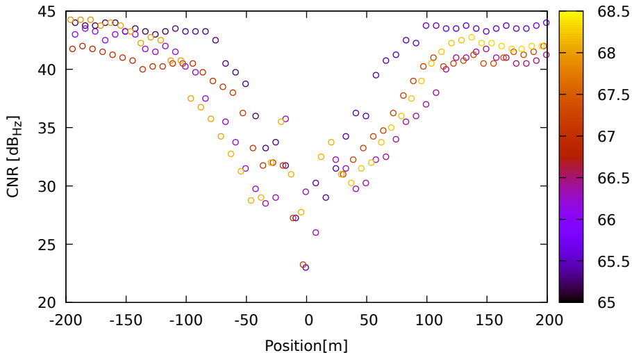
CNR vs position for G04 (L1) on SamsungS20 - DOY 263 jam. 2
