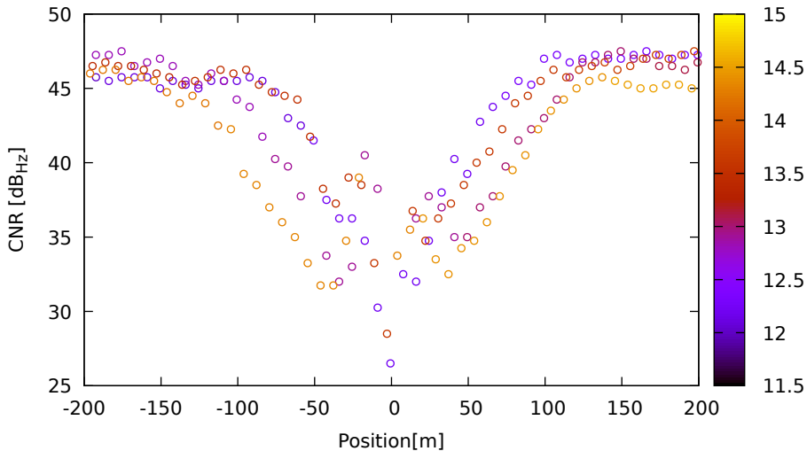
CNR vs position for G06 (L1) on SamsungS20 - DOY 263 jam. 2
