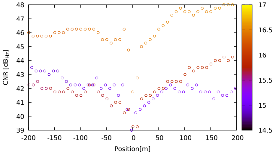
CNR vs position for G06 (L1) on SamsungS20 - DOY 263 jam. 3
