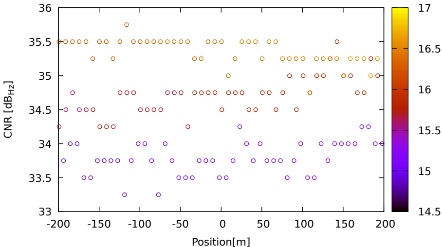
CNR vs position for G06 (L5) on SamsungS20 - DOY 263 jam. 3
