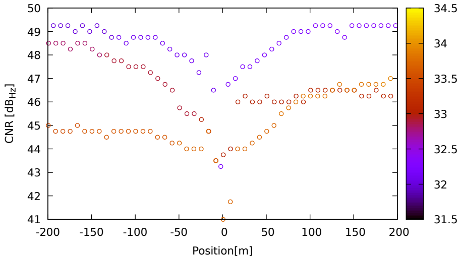
CNR vs position for G09 (L1) on SamsungS20 - DOY 263 jam. 3
