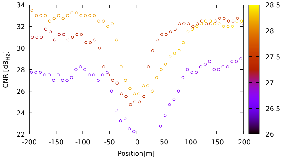
CNR vs position for G09 (L5) on SamsungS20 - DOY 263 jam. 1
