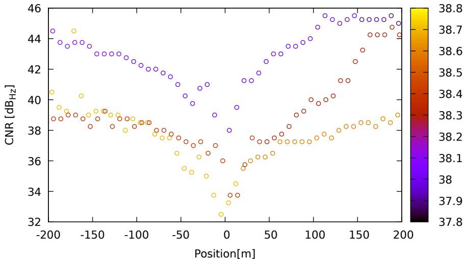
CNR vs position for G17 (L1) on SamsungS20 - DOY 263 jam. 1
