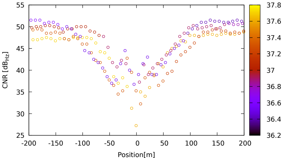
CNR vs position for G17 (L1) on SamsungS20 - DOY 263 jam. 2
