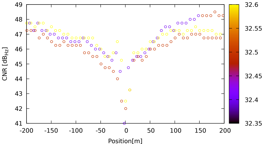
CNR vs position for G19 (L1) on SamsungS20 - DOY 263 jam. 3
