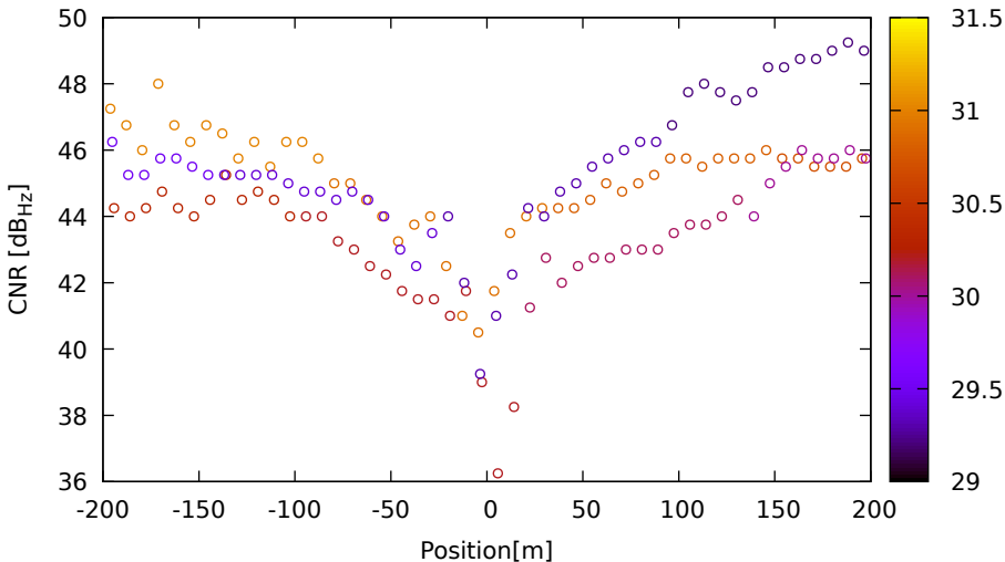
CNR vs position for G21 (L1) on SamsungS20 - DOY 263 jam. 1
