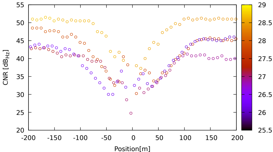
CNR vs position for G21 (L1) on SamsungS20 - DOY 263 jam. 2
