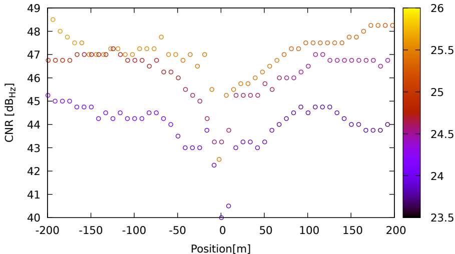
CNR vs position for G21 (L1) on SamsungS20 - DOY 263 jam. 3
