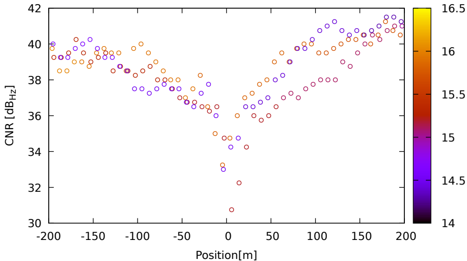
CNR vs position for G22 (L1) on SamsungS20 - DOY 263 jam. 1
