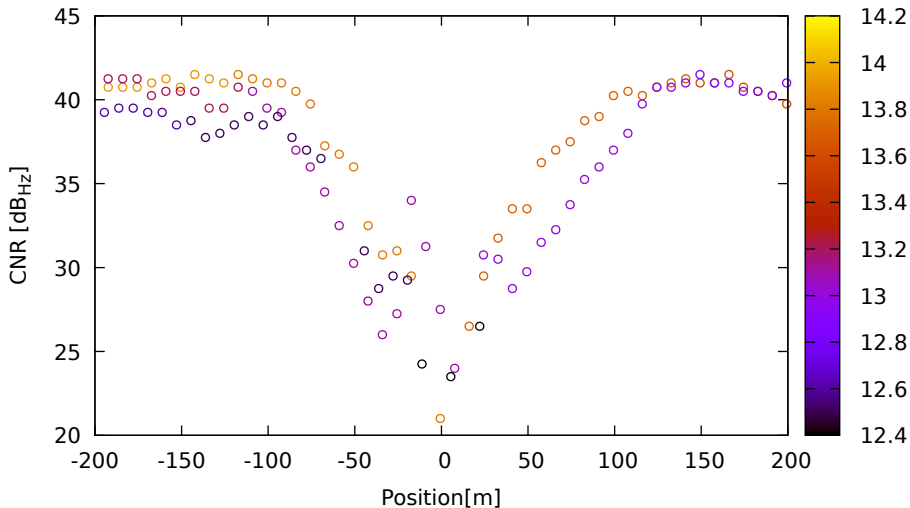
CNR vs position for G22 (L1) on SamsungS20 - DOY 263 jam. 2
