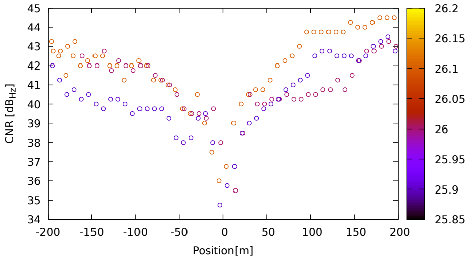
CNR vs position for G31 (L1) on SamsungS20 - DOY 263 jam. 1
