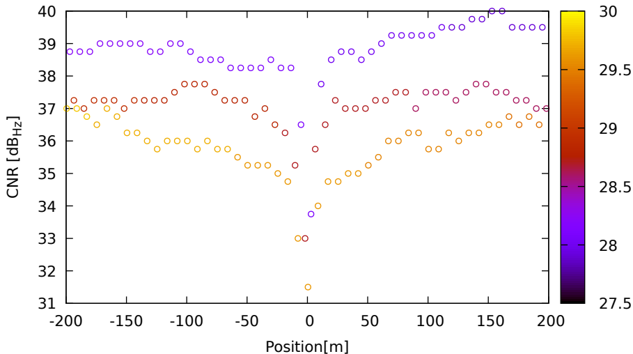
CNR vs position for C11 (B1) on Xiaomi11T - DOY 263 jam. 3
