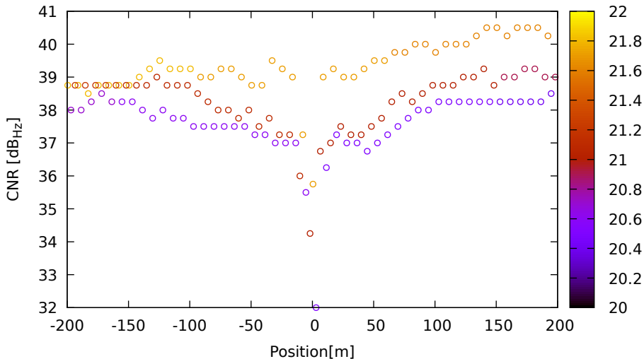
CNR vs position for C21 (B1) on Xiaomi11T - DOY 263 jam. 3
