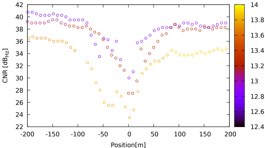
CNR vs position for C26 (B1) on Xiaomi11T - DOY 263 jam. 1
