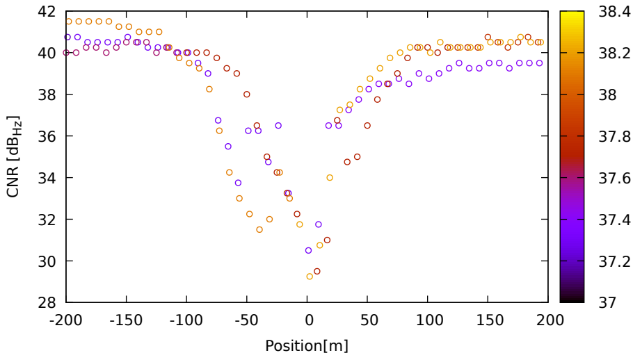
CNR vs position for C28 (B1) on Xiaomi11T - DOY 263 jam. 1
