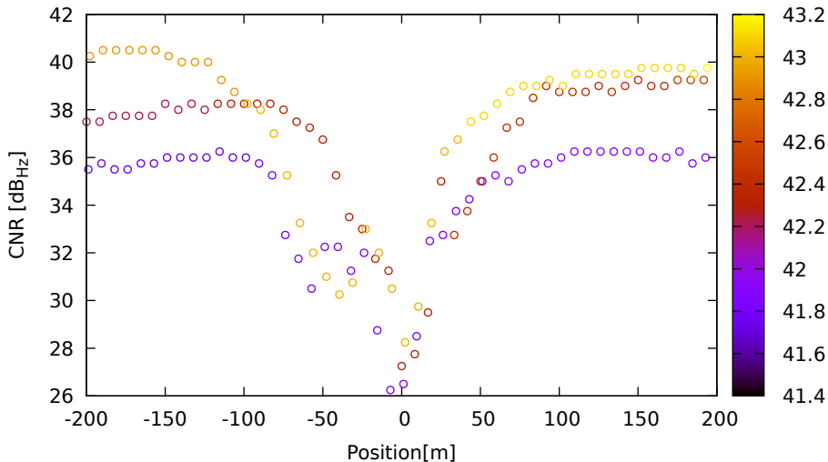
CNR vs position for C33 (B1) on Xiaomi11T - DOY 263 jam. 1
