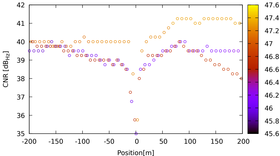
CNR vs position for C33 (B1) on Xiaomi11T - DOY 263 jam. 3
