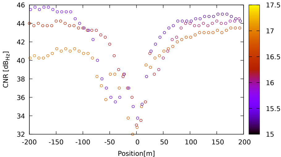
CNR vs position for C34 (B1) on Xiaomi11T - DOY 263 jam. 1
