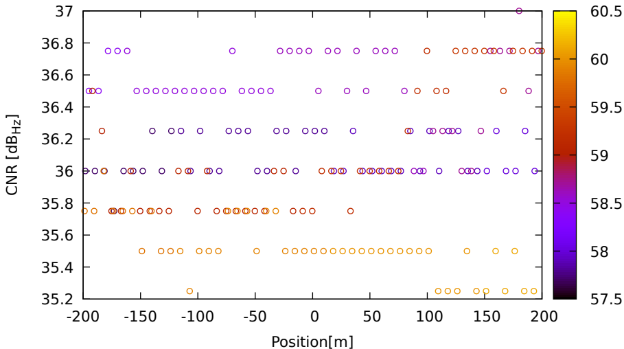
CNR vs position for E04 (E5a) on Xiaomi11T - DOY 263 jam. 2
