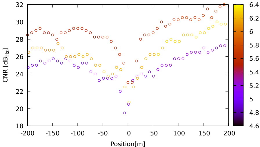
CNR vs position for E09 (E1) on Xiaomi11T - DOY 263 jam. 1
