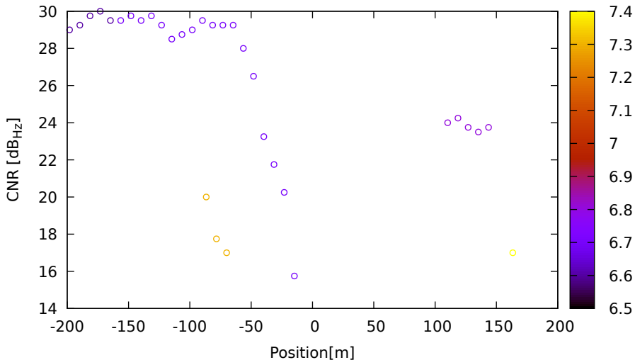
CNR vs position for E09 (E1) on Xiaomi11T - DOY 263 jam. 2
