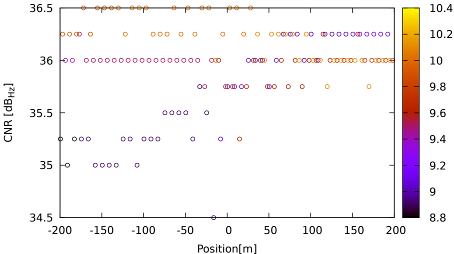
CNR vs position for E09 (E5a) on Xiaomi11T - DOY 263 jam. 3
