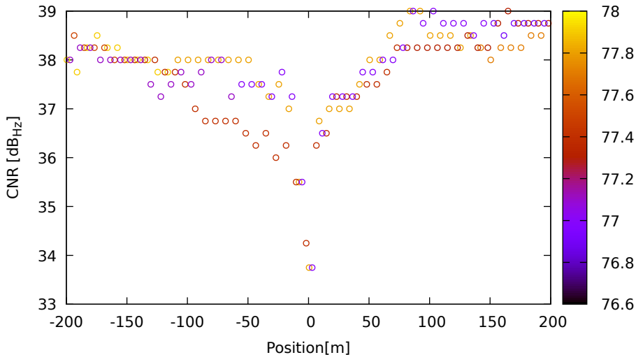
CNR vs position for E10 (E1) on Xiaomi11T - DOY 263 jam. 3
