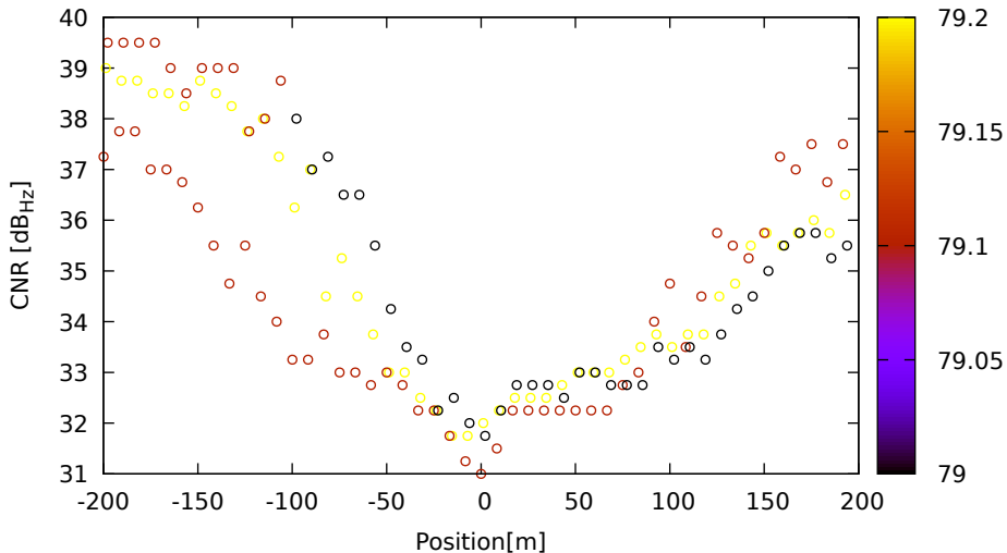
CNR vs position for E10 (E5a) on Xiaomi11T - DOY 263 jam. 1
