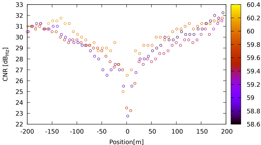
CNR vs position for E19 (E1) on Xiaomi11T - DOY 263 jam. 1
