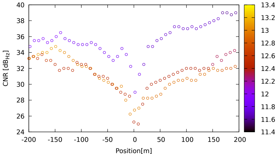
CNR vs position for E33 (E1) on Xiaomi11T - DOY 263 jam. 1
